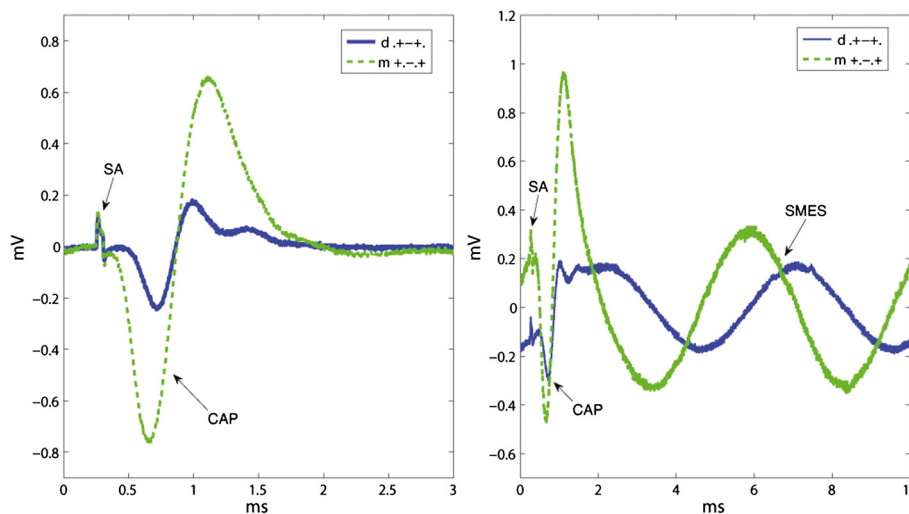
Figure 12 Recording examples that compare dot and mixed configurations. The stimulation artifacts (SAs) and compound action potentials (CAPs) appear chronologically in the left inset without the induced simulated myoelectric signal (SMES). Recordings from both configurations were obtained during the same session. Since the “end effect” was found negligible for 5 mm inwards contact displacements in our experiments, the difference in SNR can be mostly attributed to the change between ring and dot outer contacts. This resulted in an average IR(SMES) = 2.91 (m+.-.+/d.+-.+) and IR(SA) = 1.80 (m+.-.+/r.+-.+).
